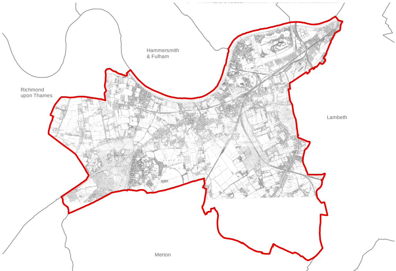
Fig.29: Historic map 1869-1874
