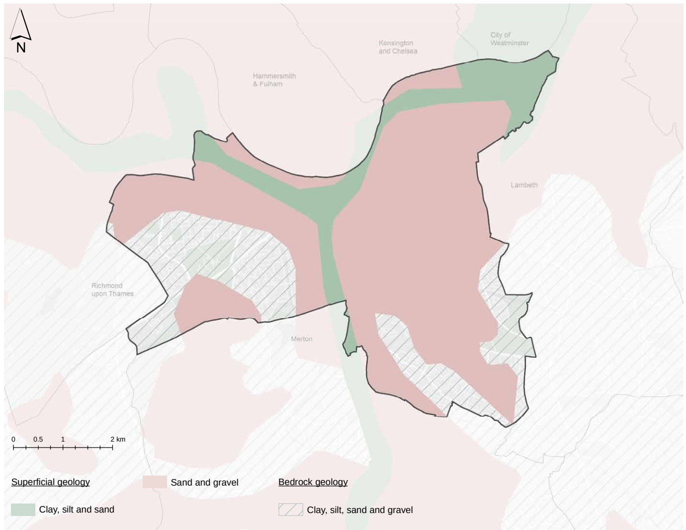
Fig. 24: Geology plan
