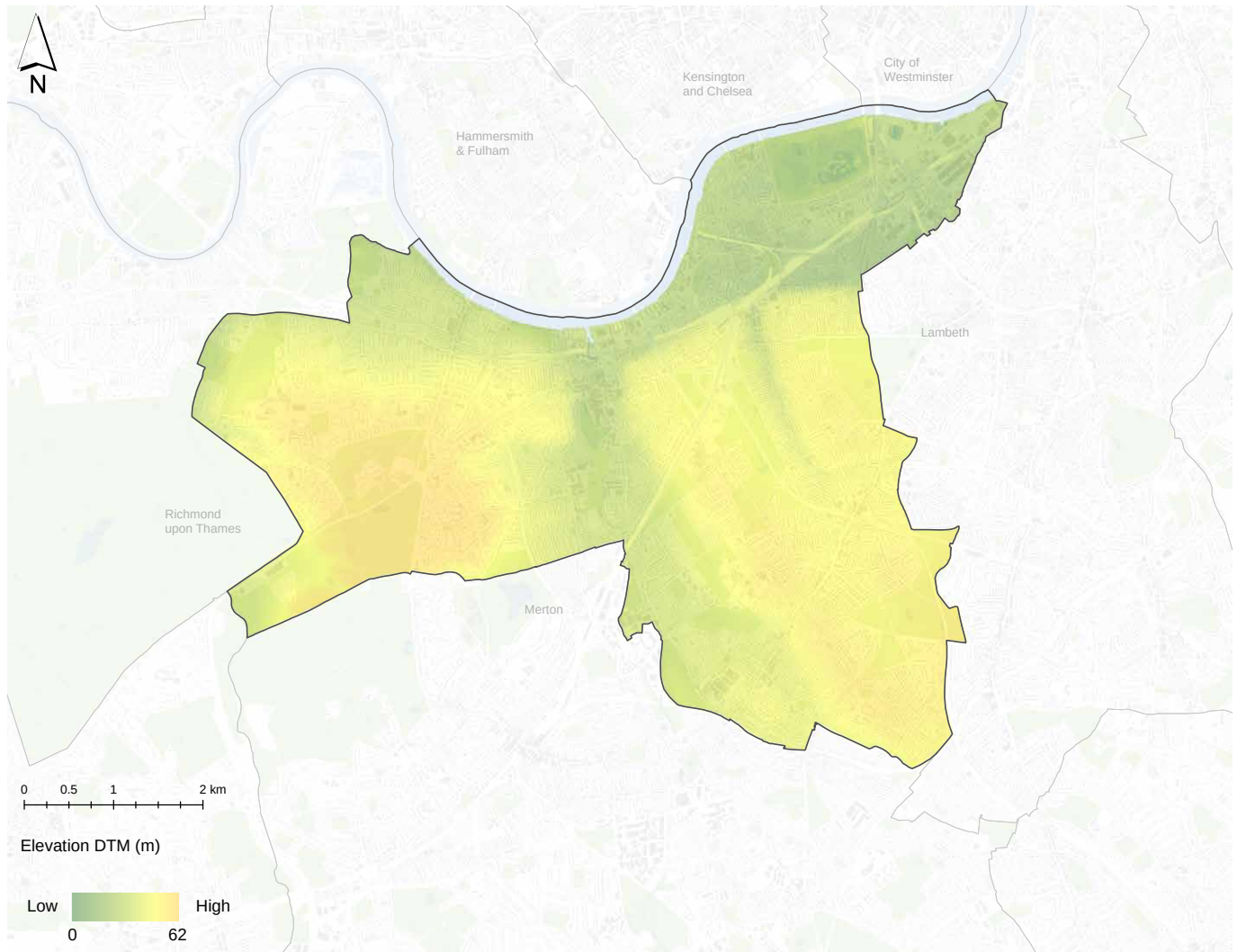
Fig.23: Topography plan
