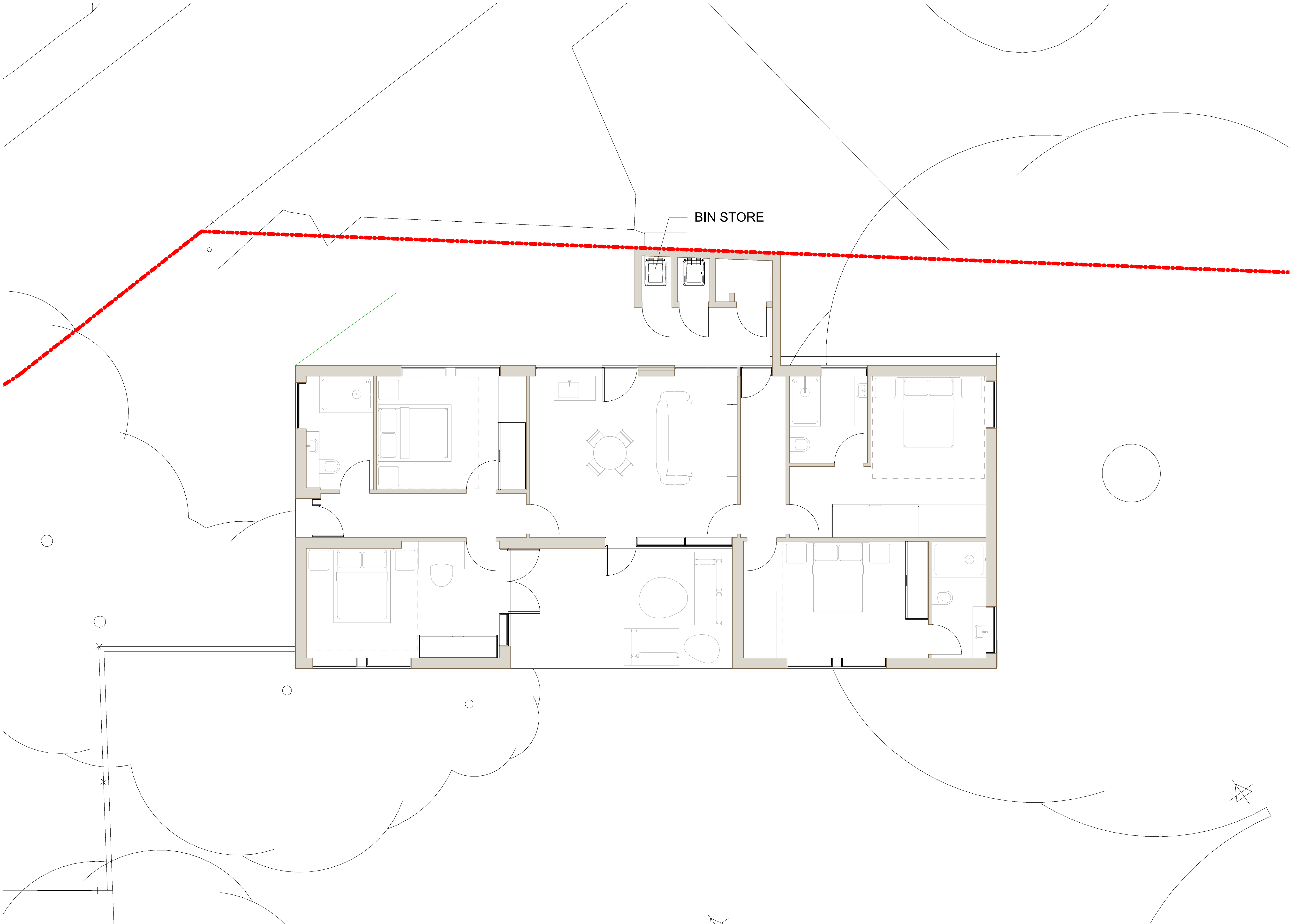
1 Proposed Bungalow - Plan 1 : 50
